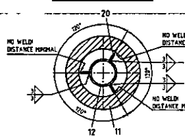
SECTION B-B SC 12
