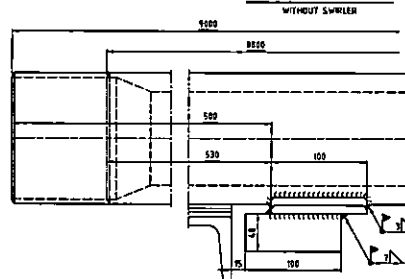
SWIRLER SC 15
