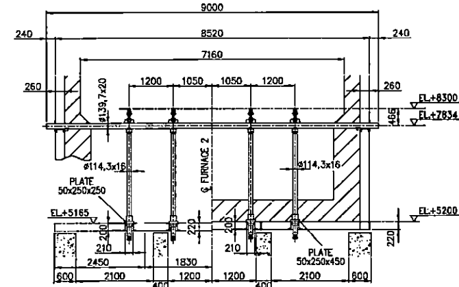
SECTION 1/2 D-D | 1/2 E-E
