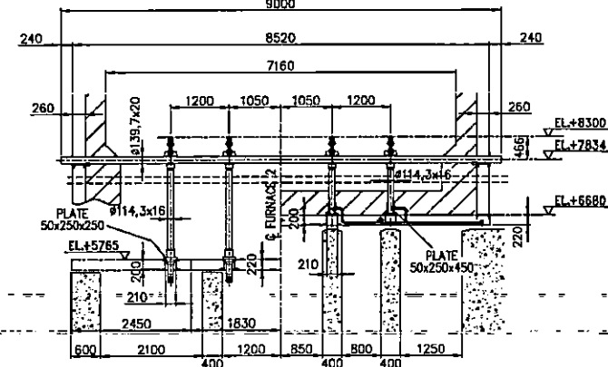
SECTION 1/2 C-C | 1/2 B-B
