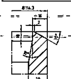
DETAIL "V" SC 11
